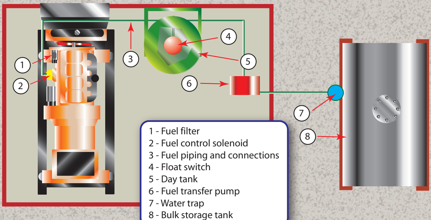
Diagram - Fuel System Maintenance Points
